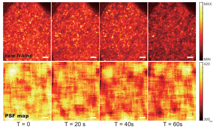
Fig. 7. Results of adaptive PSF estimation with live-cell imaging data. (top) High-density raw camera images acquired during 60 seconds, and (bottom) the widths of locally estimated PSFs in terms of FWHM. PSFs were estimated at each local patch. Scale bars are 2 \mu\text{m} in (a-d).
