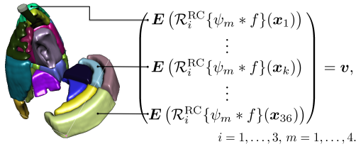
Fig. 2. Construction of the feature vector \mathbf{v} from regional averaging of the energies E(\mathcal{R}_i^{\text{RC}}\{\psi_m * f\}(\mathbf{x})) [9].
