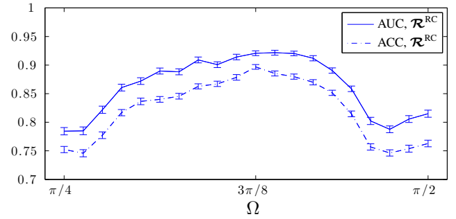
Fig. 3. Classification performance for \Omega \in [\pi/4, \pi/2] using the rotation–covariant operator \mathcal{R}^{\text{RC}} . The importance of wavelet bandwidth optimization for lung texture analysis is highlighted, where \Omega = 3\pi/8 provided best AUC=0.921 and best ACC=0.897.
