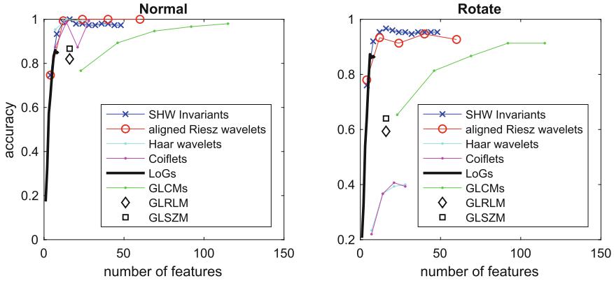
Fig. 3. Classification accuracies with respect to the number of features for both Normal and Rotate test suites. Chance level accuracy is 0.07.
