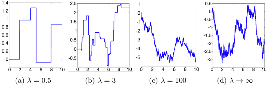
Figure 4.2: Processes whitened by D . In (a)-(c) Gauss-Poisson noises. In (d), Gaussian noise.
