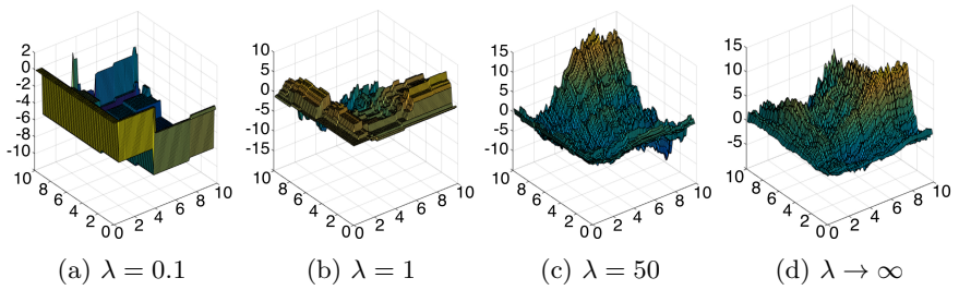
Figure 4.5: 3-D representation of the processes in Figure 4.4.
