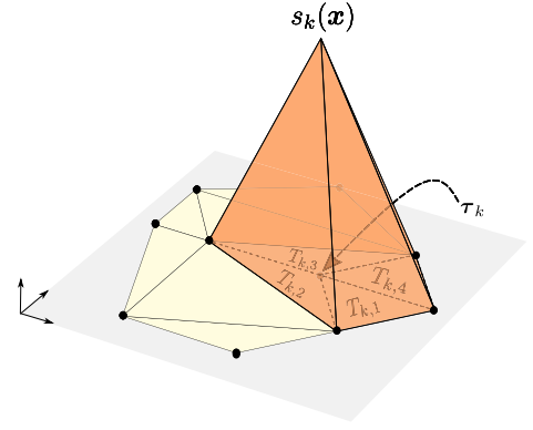
FIGURE 2. The k th vertex of the triangulation with coordinate \tau_k is included in 4 domain simplices \{T_{k,l}\}_{l=1}^4 over which the associated simplicial basis (hat) function s_k(\mathbf{x}) is illustrated.
