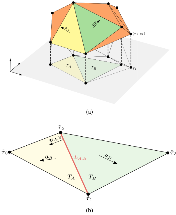
FIGURE 3. (a) Example of a CPWL function f_{\text{Hull}} defined through a triangulation. Over each simplex T_A , one can identify the function f_{\text{Hull}} by the plane that passes through the points \{(\tau_k, f_{\text{Hull}}(\tau_k) = c_k)\}_{\tau_k \in T_A} . The vector n_A corresponds to the normal vector of that plane. (b) Top view of the domain simplices T_A and T_B .
