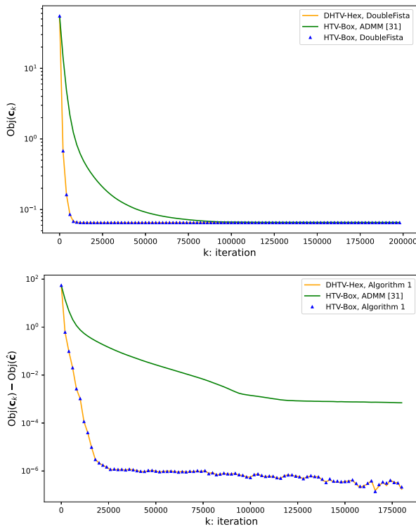
FIGURE 5. Loss of the learning task as implemented through Algorithm 1 versus the scheme used in [31].
