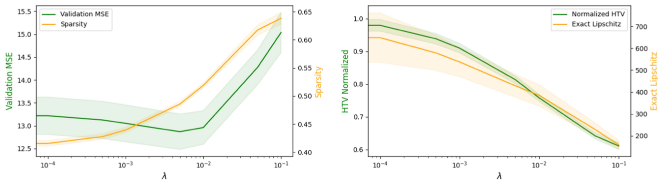
FIGURE 6. Effect of the regularization hyperparameter \lambda in the DHTV framework on: (i) average validation mean-squared error; (ii) sparsity; (iii) HTV; and (iv) Lipschitz constant for the PowerPlant dataset. The 90% confidence interval of each metric is depicted.
