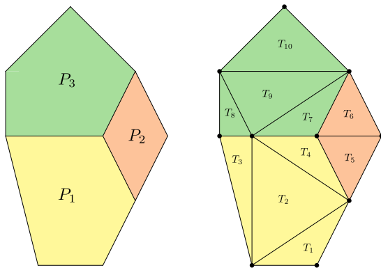
FIGURE 1. Domain of a two-dimensional CPWL function. Each patch corresponds to one linear region (left) and its partition into simplices through a Delaunay triangulation (right).
