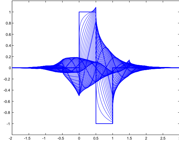
Fig. 3: The fractional B-spline wavelets with \alpha \geq 0 . These functions interpolate the conventional B-splines wavelets, which are represented using a thicker line.
