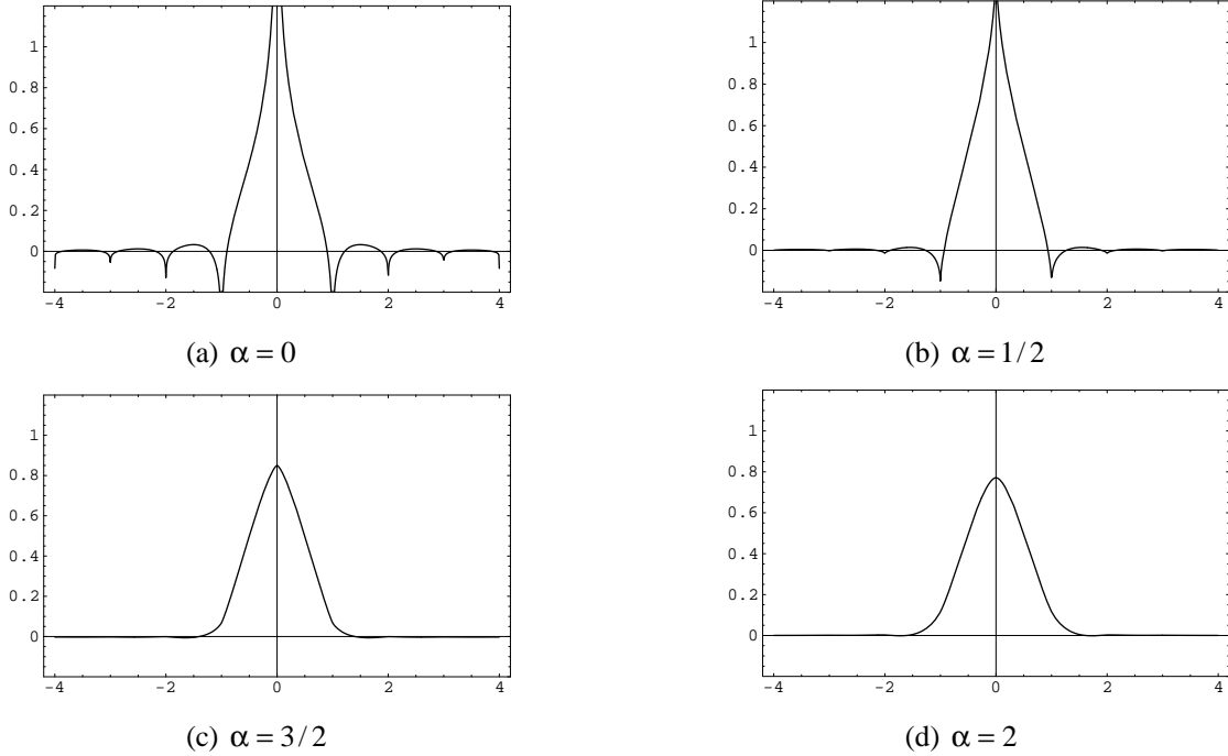
Fig. 2: Examples of symmetric fractional B-splines of increasing regularity.
