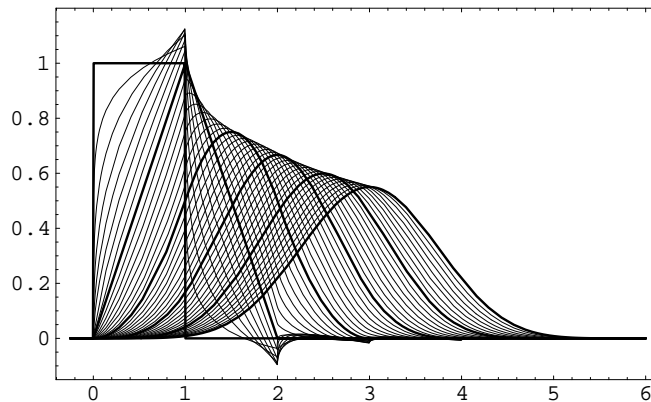
Fig. 1: The fractional B-splines with \alpha \geq 0 . These functions interpolate the conventional B-splines which are represented using a thicker line.
