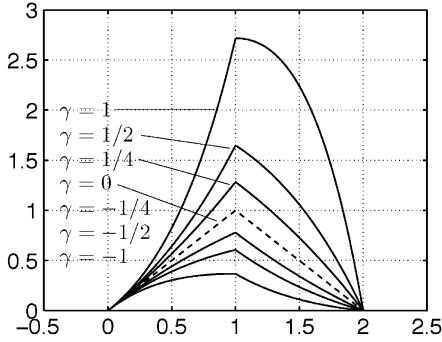
Fig. 3. Exponential B-splines \beta_{\vec{\gamma}}(t) with parameter \vec{\gamma} = [\gamma \ \gamma] , where \gamma is real. The classical second-order B-spline (the triangle function in dashed lines) is obtained for \gamma = 0 .
