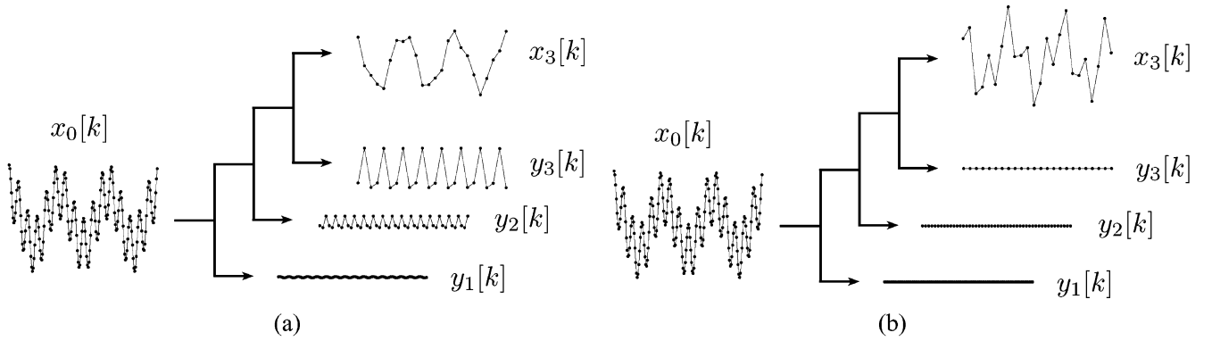
Fig. 1. Three-level discrete orthonormal wavelet transforms of a signal with two harmonic components ( x_0[k] = \cos(k\pi/32) + \cos(k\pi/6) ). The wavelet coefficients are y_1[k] , y_2[k] , and y_3[k] ; x_3[k] contains the scaling function coefficients at the coarsest level. (a) Using 8-tap Daubechies filters (corresponding to \vec{\alpha} = [0 \ 0 \ 0 \ 0] in Section IV-B). (b) Using scale-dependent 8-tap generalized Daubechies filters (corresponding to \vec{\alpha} = [i\pi/32 \ -i\pi/32 \ i\pi/6 \ -i\pi/6] ).
