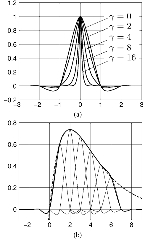
Fig. 6. (a) Interpolation functions at scale j = 0 for \vec{\gamma} = [\gamma \ \gamma \ -\gamma \ -\gamma] . (b) Reproduction of the exponential polynomial te^{-t/2} (dashed line) for \gamma = 1/2 ; the thick continuous line represents the sum in (8) truncated to k = 0 \dots 6 , while its individual terms are shown as thin lines.
