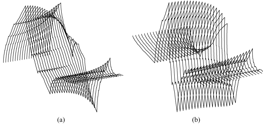
Fig. 7. Orthonormal scaling functions (a) and wavelets (b) at scale j = 0 , corresponding to \vec{\alpha} = [i\omega_0 \ -i\omega_0] , for \omega_0 = 0, \pi/32, 2\pi/32, \dots, 20\pi/32 . The classical Daubechies functions are the leftmost ones and are obtained for \omega_0 = 0 .
