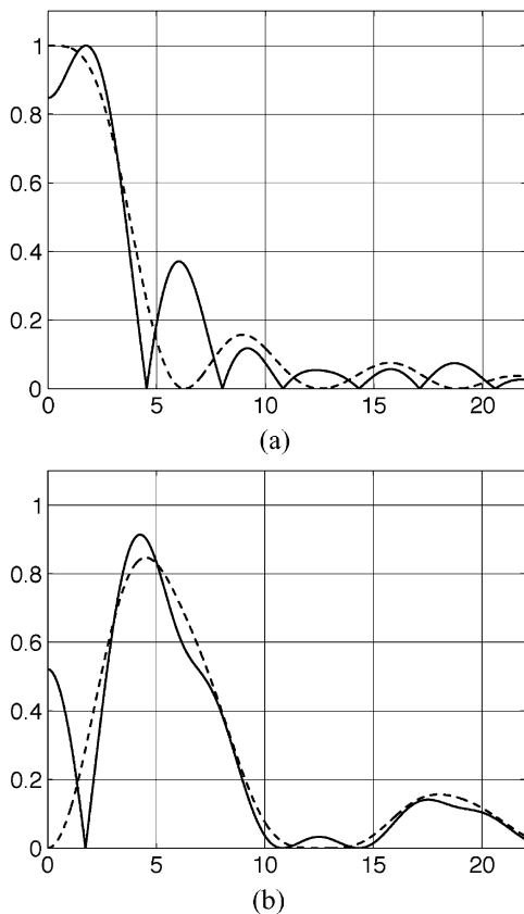
Fig. 8. Moduli of the Fourier transforms of the orthonormal scaling functions (a) and wavelets (b) at scale j = 0 , corresponding to \vec{\alpha} = [i\omega_0 \ -i\omega_0] . The classical Daubechies functions are obtained for \omega_0 = 0 and are shown as dashed lines; their generalized counterparts are shown as continuous lines, for \omega_0 = 5\pi/9 .
