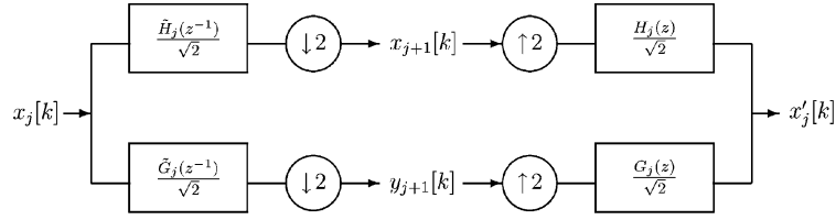
Fig. 2. Nonstationary perfect-reconstruction filter bank.
