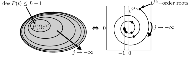
Fig. 4. Illustration of Theorem 1. For the exponential polynomials to lie in the linear span of the functions (\varphi_{j,k})_{k \in \mathbb{Z}} at all scales j , the scaling filters H_j(z) must have roots located along a logarithmic spiral converging towards -1 in the complex plane.
