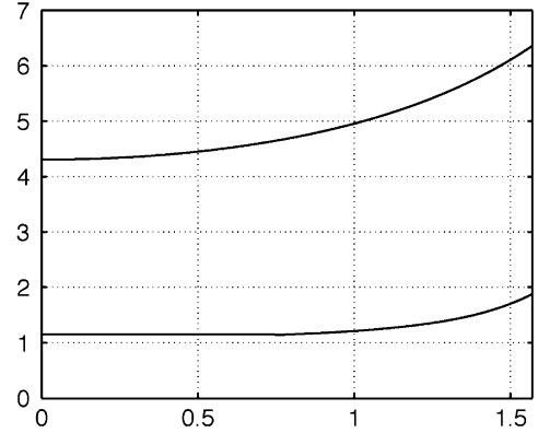
Fig. 12. Ratios of the Riesz bounds B_{20}/B_{10} for Cohen–Daubechies–Feauveau (top) and 9/7 (bottom) synthesis scaling functions at scale 0, as a function of \omega_0 ( \vec{\alpha} = \vec{\alpha} = [i\omega_0 \ i\omega_0 \ -i\omega_0 \ -i\omega_0] ).
