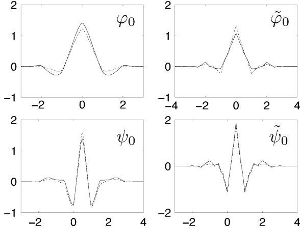
Fig. 11. Biorthogonal scaling functions and wavelets at scale 0, corresponding to a generalization of the 9/7 filters (see text). From left to right and top to bottom: \varphi_0 , \tilde{\varphi}_0 , \psi_0 and \tilde{\psi}_0 . The functions obtained from the classical 9/7 filters are represented using dashed lines.
