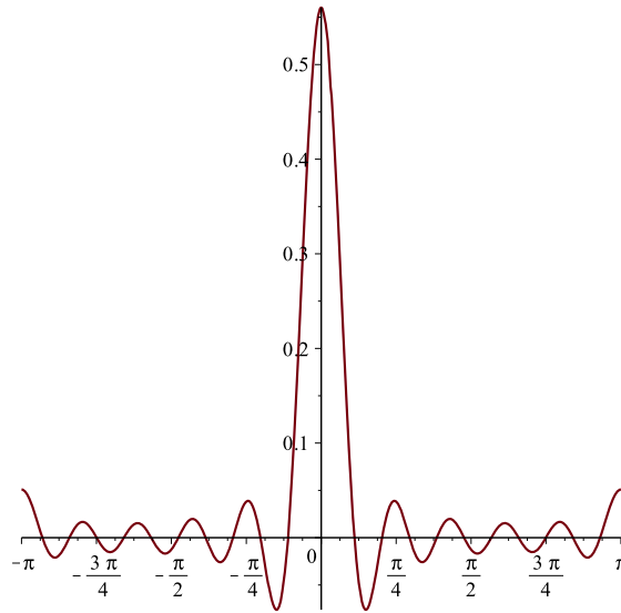
Fig. 2. Plot of the kernel A_{\ell_{max}}(\cos(\cdot)) for \ell_{max} = 10 and n_{max} = 216 .
