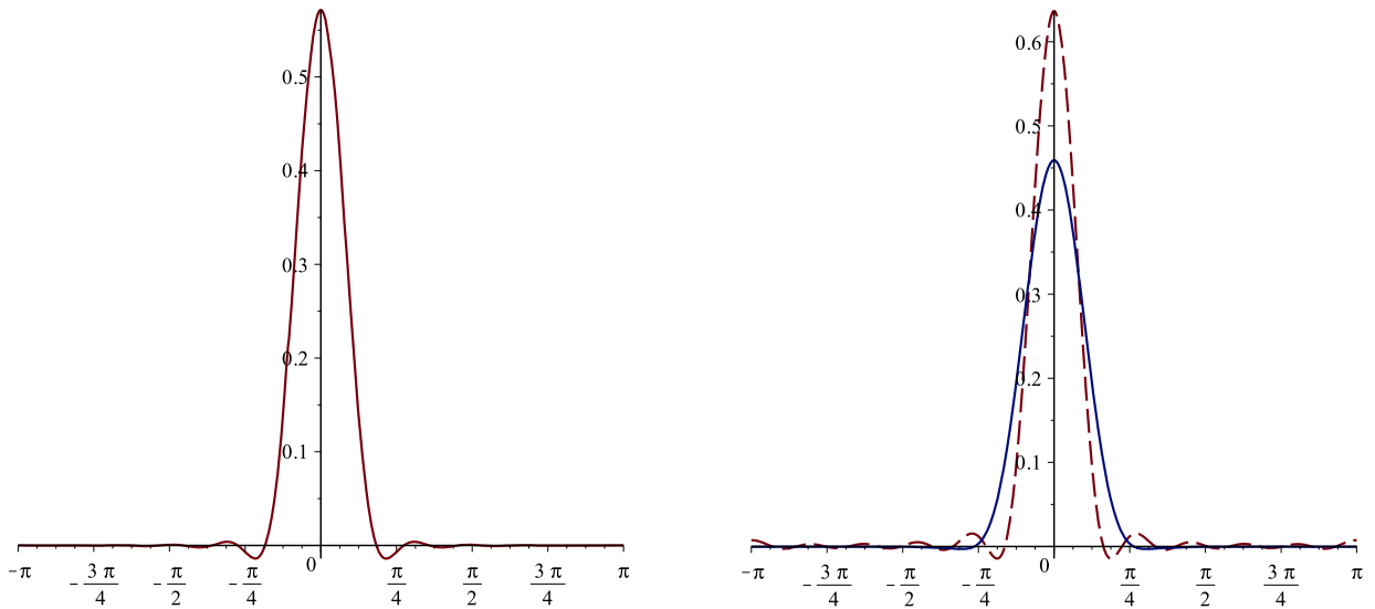
Fig. 1. Plot of zonal kernels \Lambda(\cos(\cdot)) for d = 3 , \ell_{\max} = 10 , and n_{\max} = 216 . The kernel on the left was constructed using \hat{a} from (7), while the functions on the right were constructed by choosing \hat{a} to be B-splines. In the plot on the right, the dashed line corresponds to a linear B-spline, and the solid line corresponds to a cubic B-spline.
