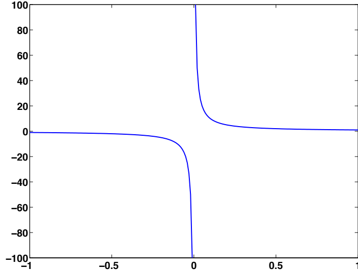
Fig. 2. The convolution kernel of the Hilbert transform, 1/\pi x . It has a singularity at the origin and its tails decay slowly. The former pathology can be overcome provided that the signal on which the transform is applied is sufficiently smooth, while the slow decay can be overcome if the signal is of compact support, or at least, of sufficient decay.
