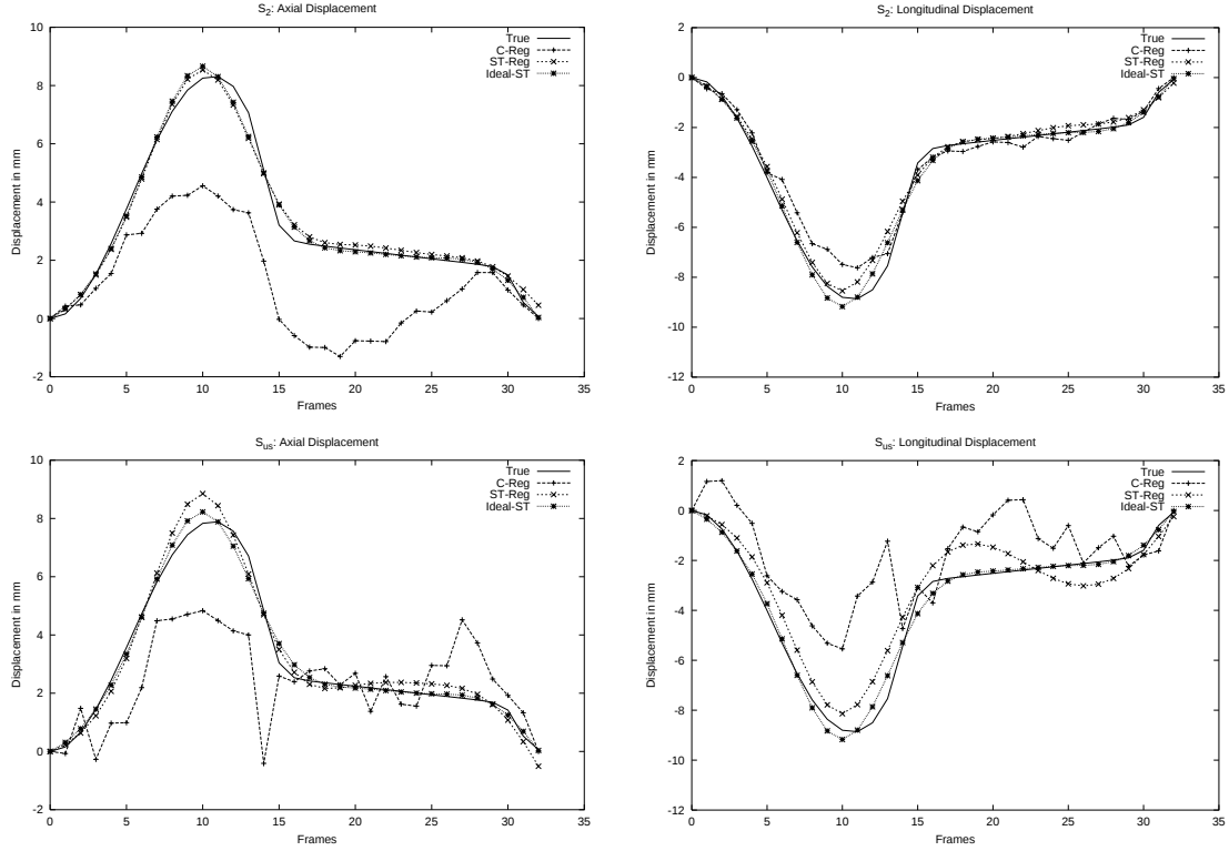
Fig. 5. Axial ( left ) and longitudinal ( right ) displacements (in millimeters) for a middle-septum point in sequences S_2 ( top ) and S_{us} ( bottom ). We show the true displacement, the displacement found by the two algorithms, and the best achievable result within the frame of the motion model used in the constrained algorithm.
