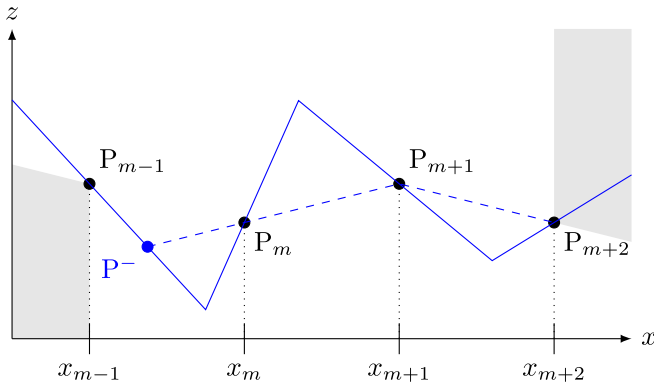
FIGURE 5. Illustration of Lemma 1 in the case a_m > 0 and a_{m+1} < 0 . The interpolant f (solid line) satisfies s^+ > s_{\text{cano}}^+ and s^- \leq s_{\text{cano}}^- . The modified interpolant \tilde{f} (dashed line) also has three knots P^- , P_{m+1} , and P_{m+2} , but none in (x_m, x_{m+1}) .
