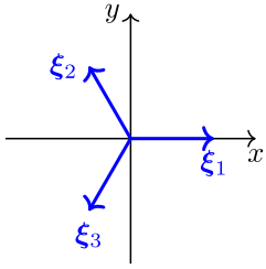
FIGURE 2. Hexagonal box-spline vectors.
