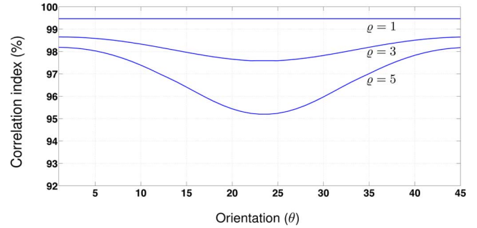
Fig. 8. Normalized correlation between the optimal four-directional box spline and the target Gaussian at different elongations and orientations. For a fixed elongation, the correlation is minimum at the critical orientation \theta = 22.5^\circ , and improves symmetrically as \theta approaches the principal orientations (see Fig. 6).
