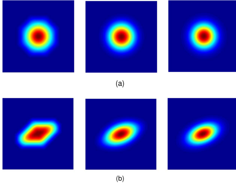
Fig. 9. Higher-order box splines through iterative convolutions. Left: The reference four-directional box spline; Center: Iterated box spline obtained by convolving the (rescaled) four-directional box spline with itself; Right: Target Gaussian having identical covariance. (a) Isotropic forms ( s = 1, d = 1 ), (b) Anisotropic forms ( s = 1, d = 3, \theta = \pi/8 ).
