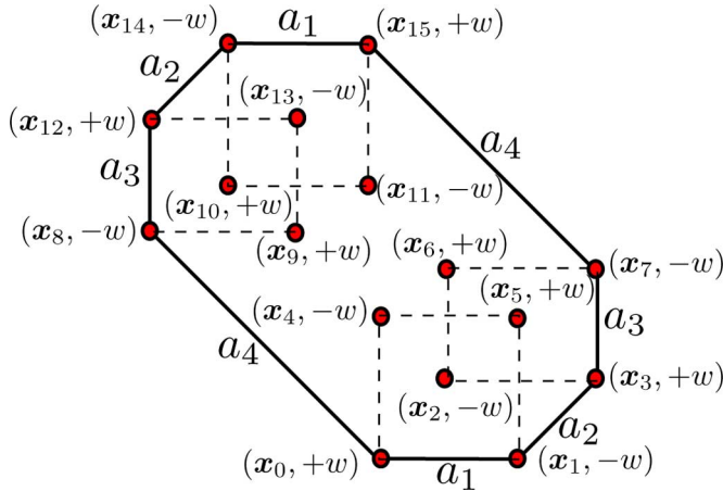
Fig. 5. Distribution of the taps of the FD mesh. The pairs (u, v) denote the positions (u) and the corresponding weights (v) of the taps of the FD mesh.
