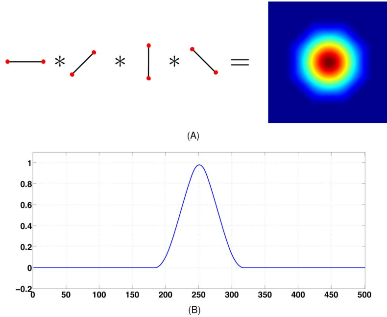
Fig. 3. Construction of the radially-uniform box spline through the convolution of four directional box distributions. (A) The four box distributions, distributed uniformly over [0, \pi) , were assigned equal scales in this example; (B) Scan profile along \theta = \pi/8 . (A) Four-directional box spline, (B) Scan profile along \theta = \pi/8 .
