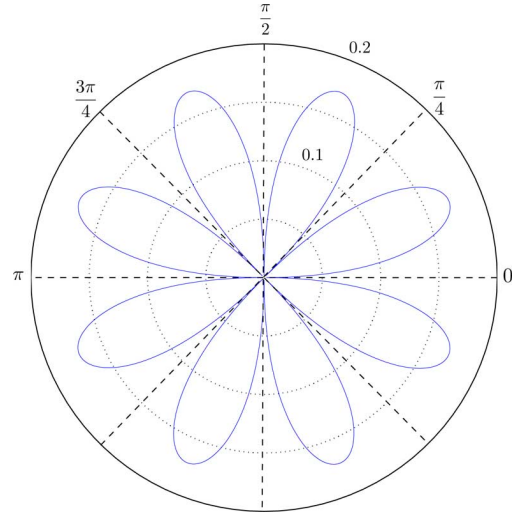
Fig. 6. Polar plot of the symmetric variation of 1/U(\phi) as a function of the filter orientation \phi , where U(\phi) is the bound on the elongation. The bound reaches its minimum when the orientation of the filter is exactly midway between two principal axes, whereas arbitrary elongation is achievable in the neighborhood of the four principal directions \phi = 0, \pi/4, \pi/2 and 3\pi/4 .
