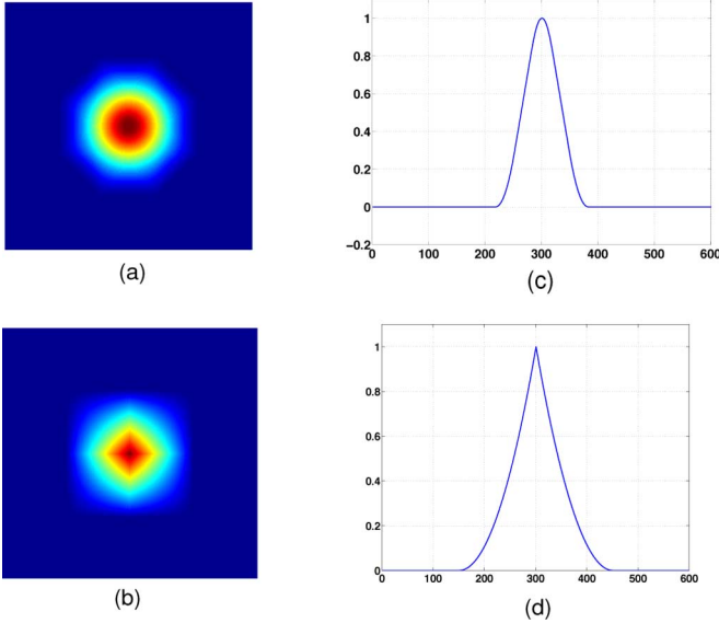
Fig. 4. Intensity distribution of (a) the radially-uniform box spline, and (b) the separable B-spline, of same order. The respective scan profiles along \pi/8 are shown in (c) and (d).
