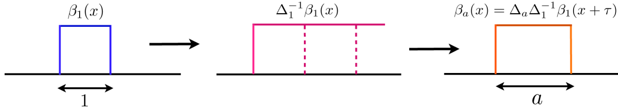
Fig. 2. Box function rescaling through “addition and subtraction” of the unit box function: The step function is first reproduced from the unit box using the running-sum, and then the appropriate finite-difference is applied to recover the rescaled box function.
