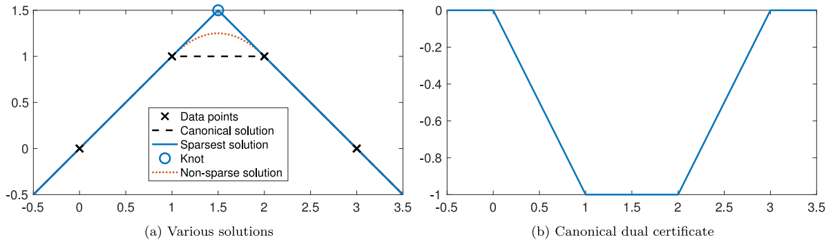
Fig. 3. Example with M = 4 of a non-unique solution ( \eta_{\text{cano}} saturates at -1 ). An example of a non-sparse solution with a quadratic regime in [1, 2] is given.
