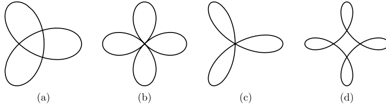
Fig. 7. Hypotrochoid curves.
