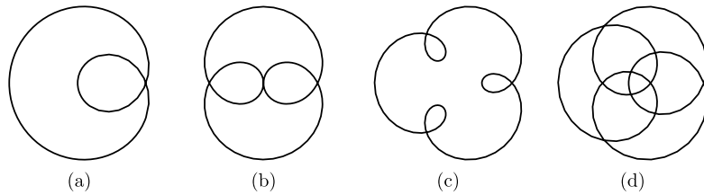
Fig. 8. Epitrochoid curves.
