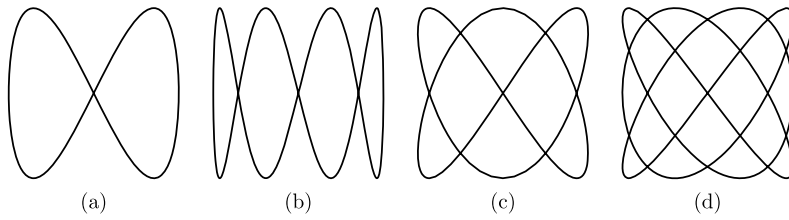
Fig. 6. Lissajous curves.
