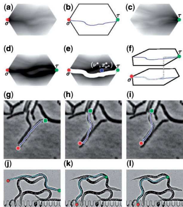
Fig. 1. Algorithm for finding the second best path. (a) Forward derived cost map (from source node \sigma ), (b) shortest path, (c) backward derived cost map (from target node \tau ), (d) summed cost map, (e) exclusion corridor mask and node (\nu^*, x_{\nu^*}^*) with minimal cost and (f) resulting second shortest path obtained by backtracking paths from (\nu^*, x_{\nu^*}^*) to \sigma and \tau . The underlying input image, source and target locations are those shown in (k). Application examples in images of mycobacteria (phase-contrast) and nematodes (bright-field). For some objects, the shortest path corresponds to the desired one [(g) and (j)], but for others in the same image [(h) and (k)], only the M th shortest is correct [(i) and (l)]
