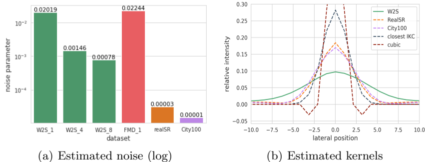
Fig. 2: Noise and kernel estimation on images from different datasets. A comparably-high noise level and a wide kernel indicate that the HR images of W2S are challenging to recover from the noisy LR observation.
