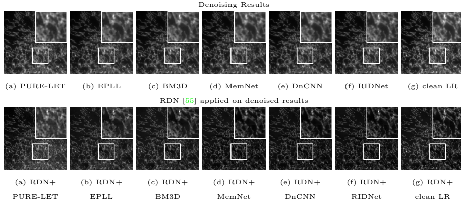
Fig. 3: The first row shows qualitative results of the denoising algorithms on a test LR image with the highest noise level. The second row shows qualitative results of the SR network RDN [55] applied on top of the denoised results. RDN amplifies the artifacts created by PURE-LET and EPLL, and is unable to recover faithful texture when the input image is over-smoothed by denoising algorithms. A gamma correction is applied for better visualization. Best viewed on screen.
